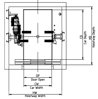
HOISTWAY PLAN
